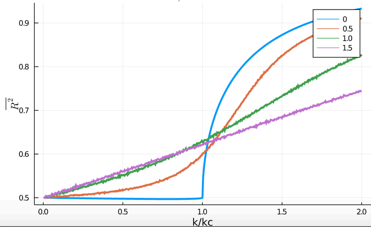
\overline{R^2} vs. k/k_c for Several \sigma
